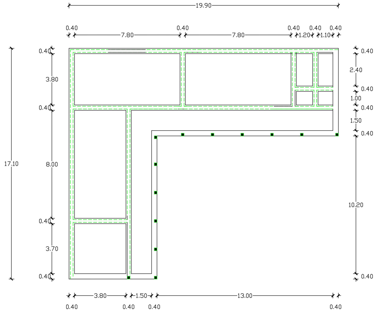
FOUNDATION PLAN (CLASS ROOMS)
